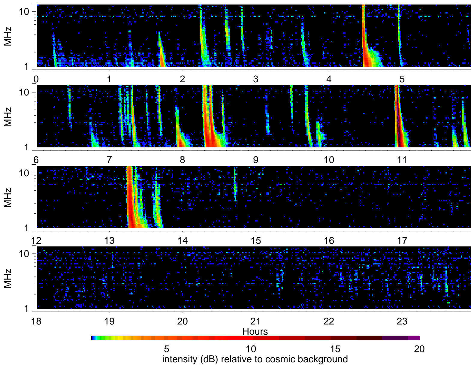
Wind Waves RAD2 receiver: 2000/11/18
