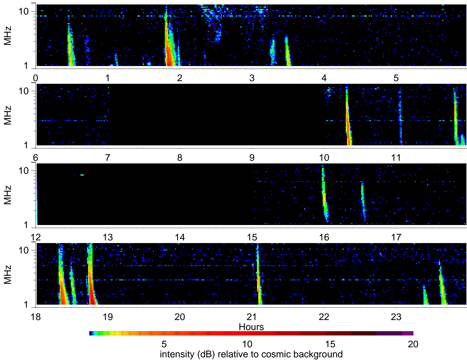
Wind Waves RAD2 receiver: 2000/11/16
