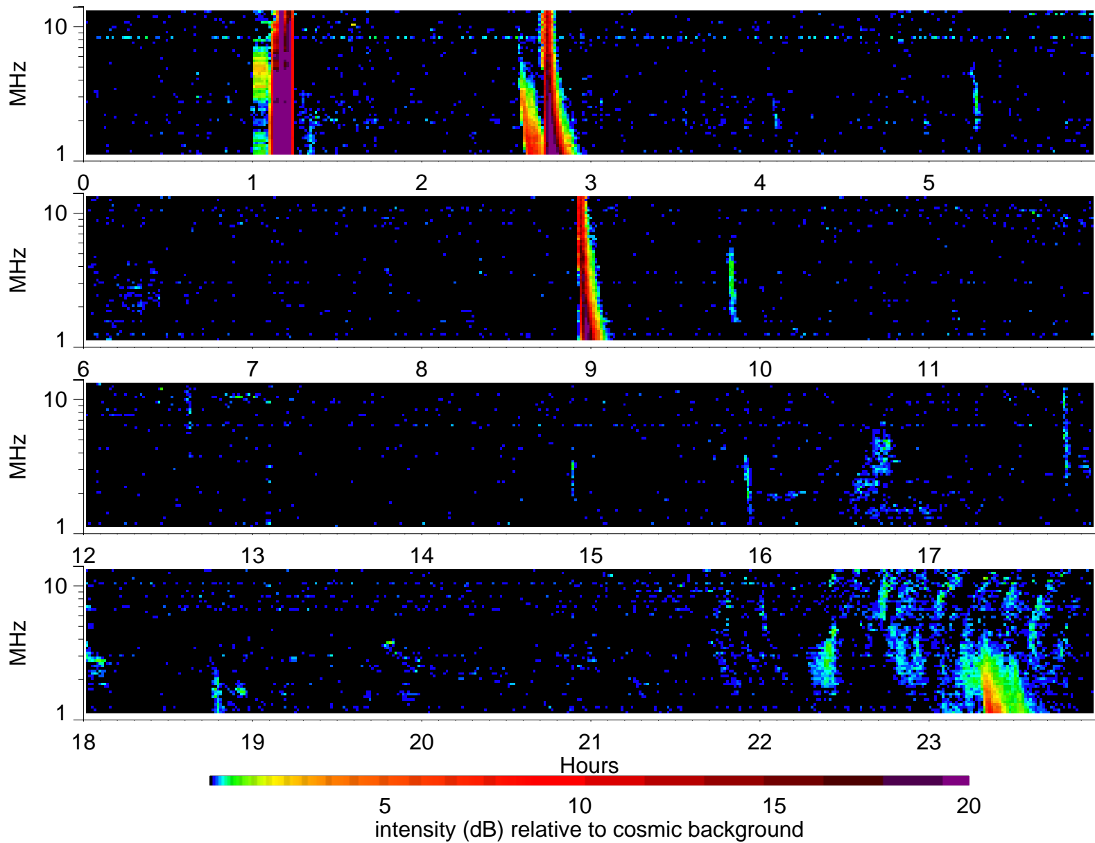
Wind Waves RAD2 receiver: 2000/11/15
