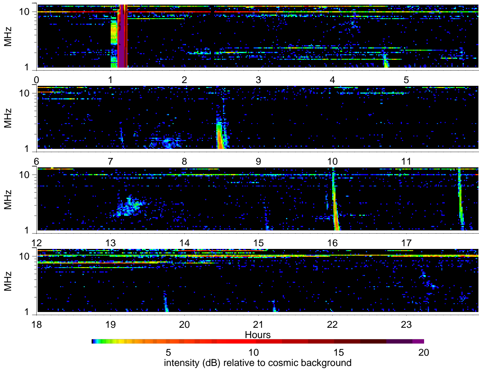
Wind Waves RAD2 receiver: 2000/11/11
