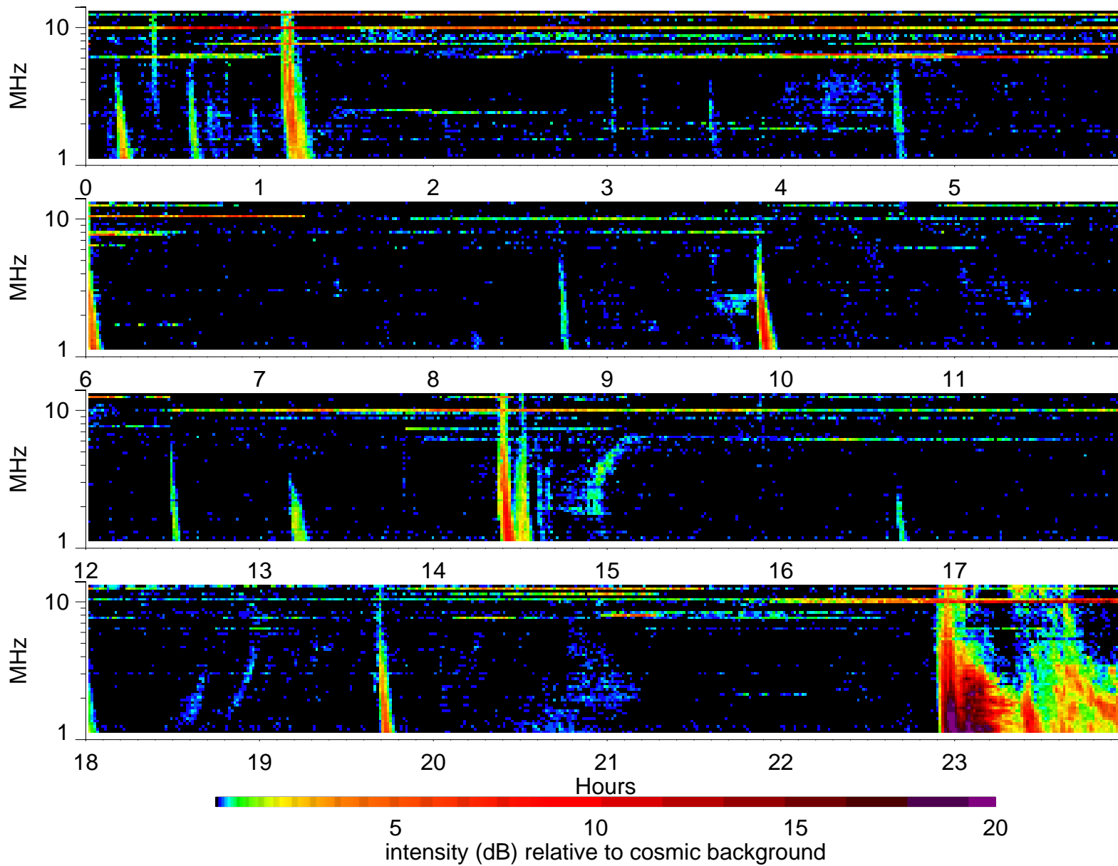
Wind Waves RAD2 receiver: 2000/11/8
