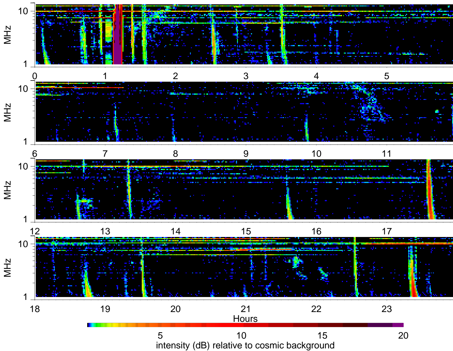
Wind Waves RAD2 receiver: 2000/11/5
