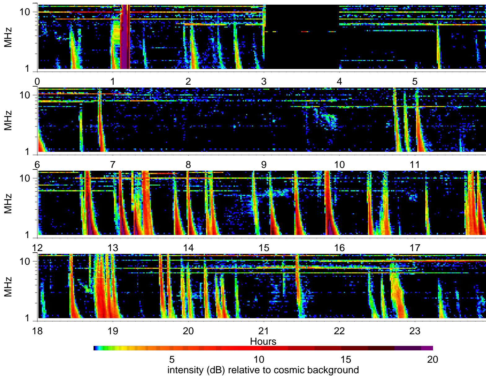
Wind Waves RAD2 receiver: 2000/11/3
