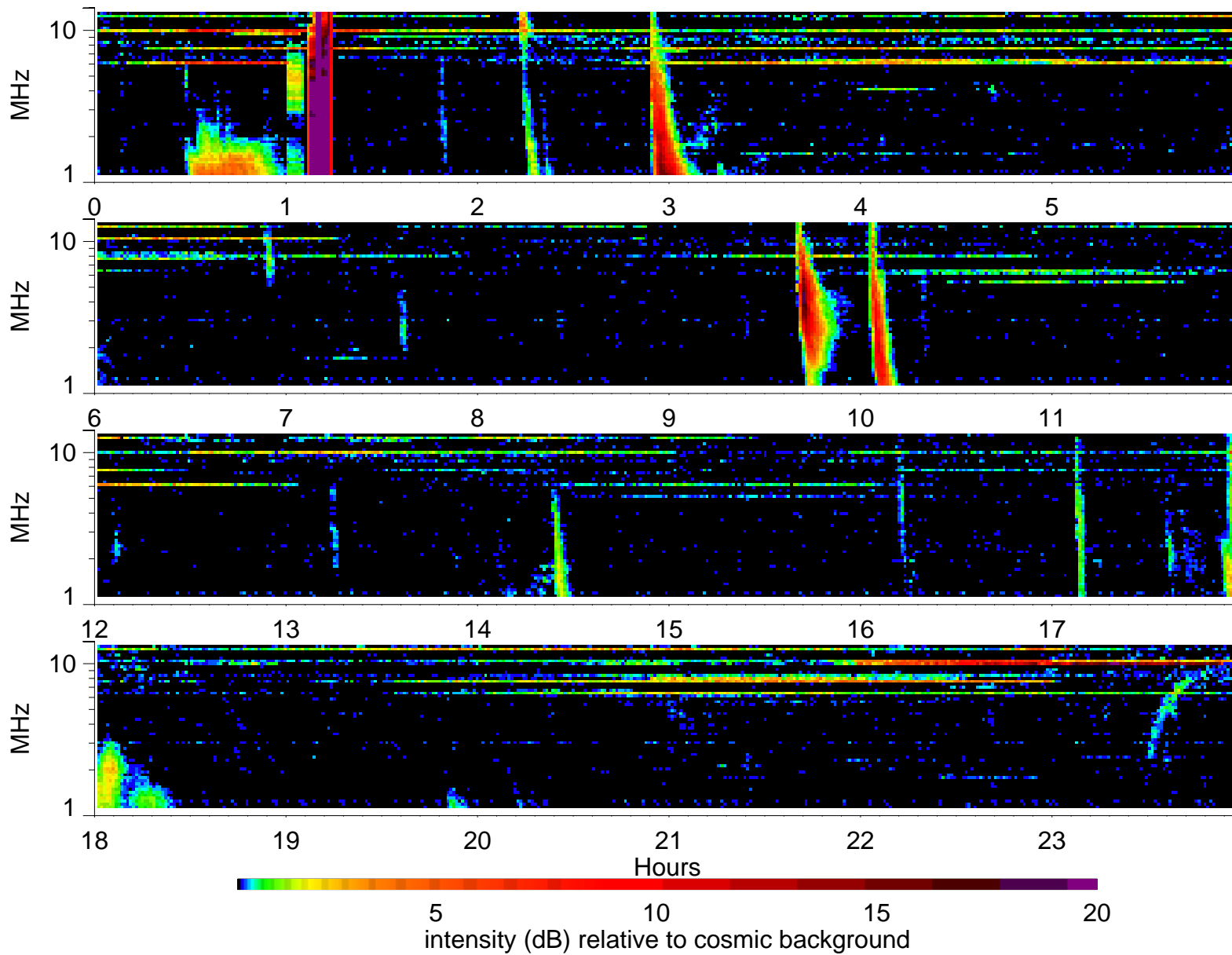
Wind Waves RAD2 receiver: 2000/10/30
