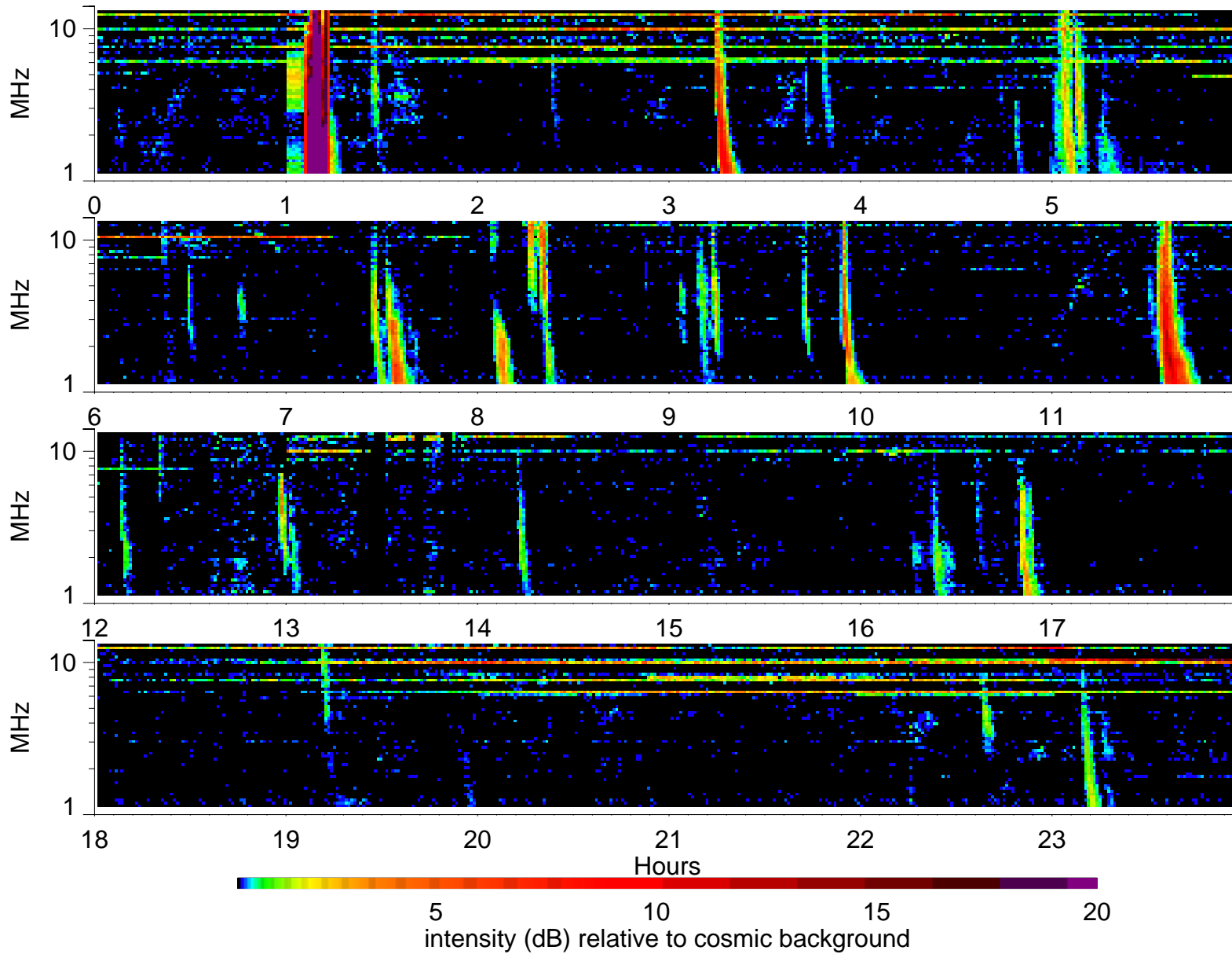
Wind Waves RAD2 receiver: 2000/10/26
