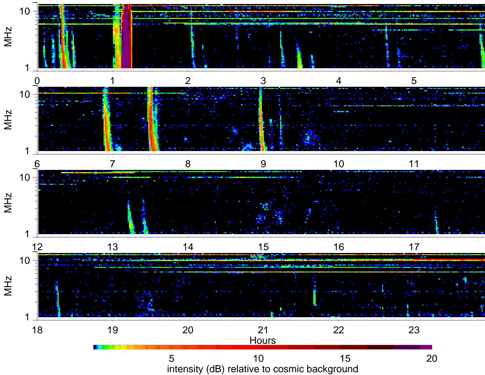
Wind Waves RAD2 receiver: 2000/10/20
