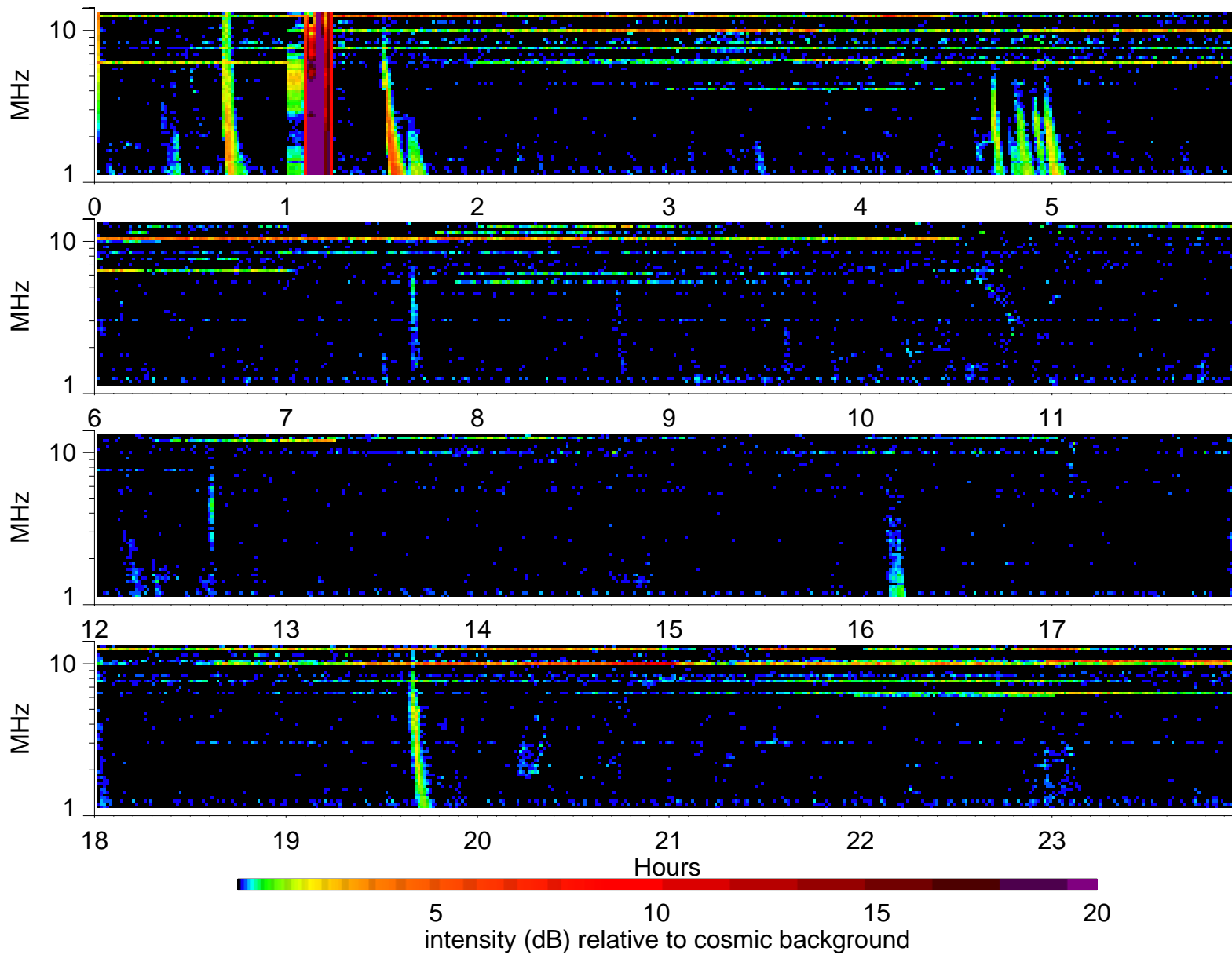
Wind Waves RAD2 receiver: 2000/10/14
