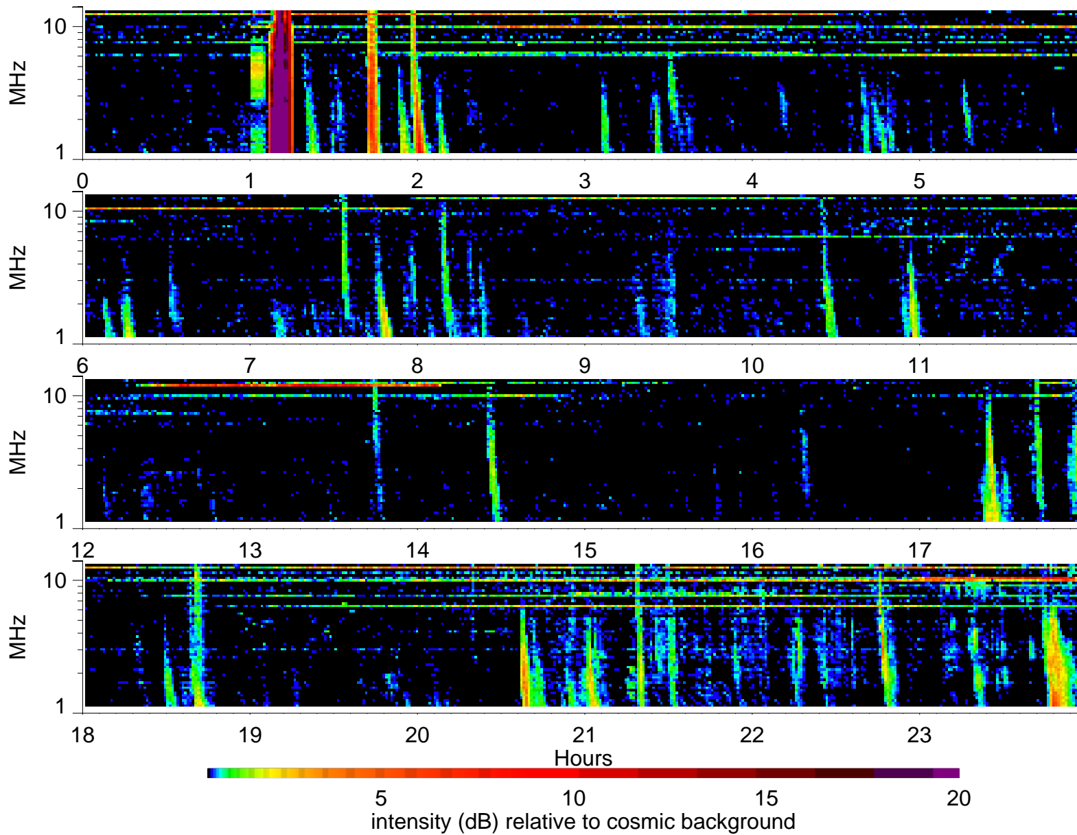
Wind Waves RAD2 receiver: 2000/10/12
