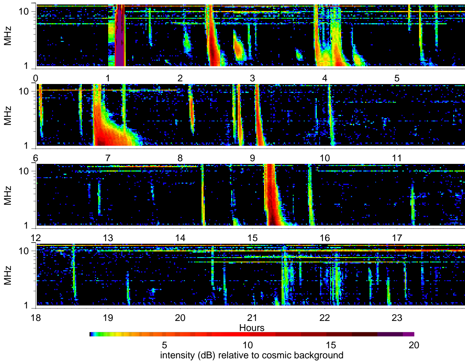
Wind Waves RAD2 receiver: 2000/10/10
