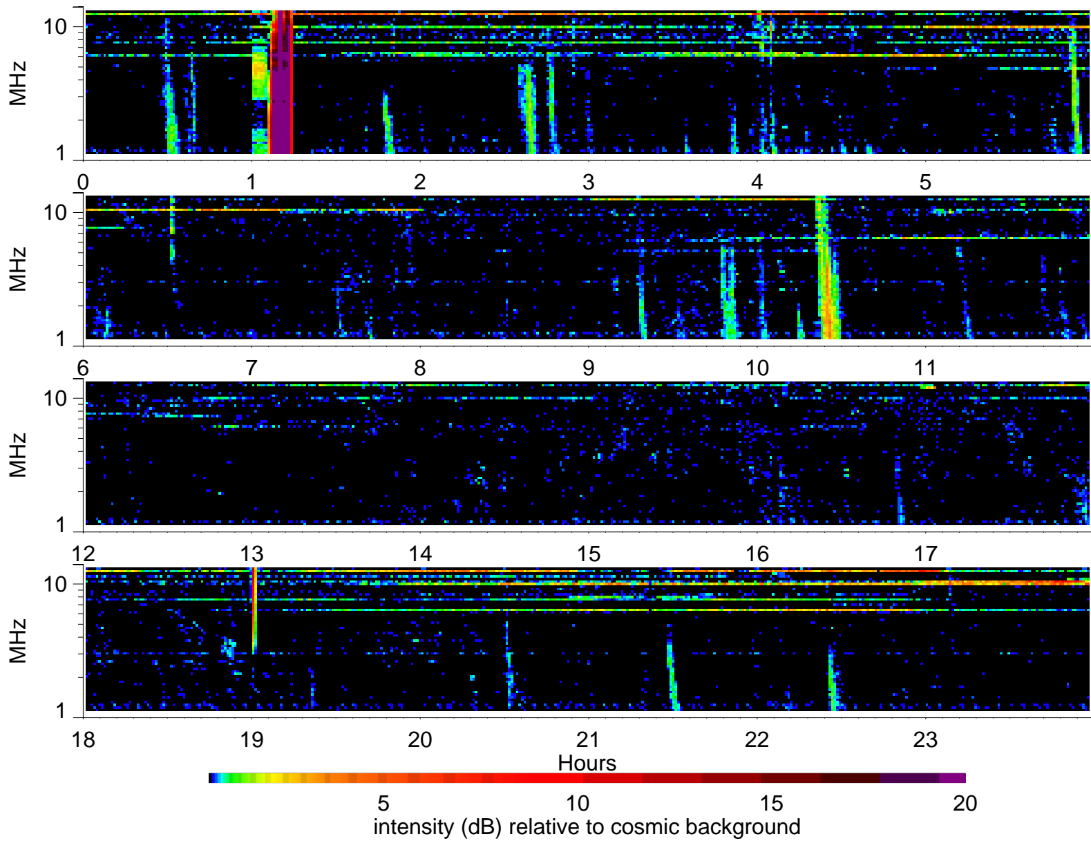
Wind Waves RAD2 receiver: 2000/10/8
