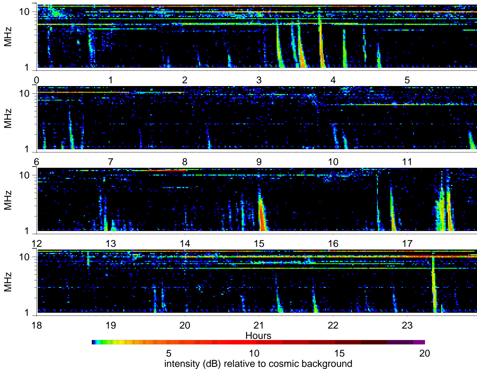
Wind Waves RAD2 receiver: 2000/10/7
