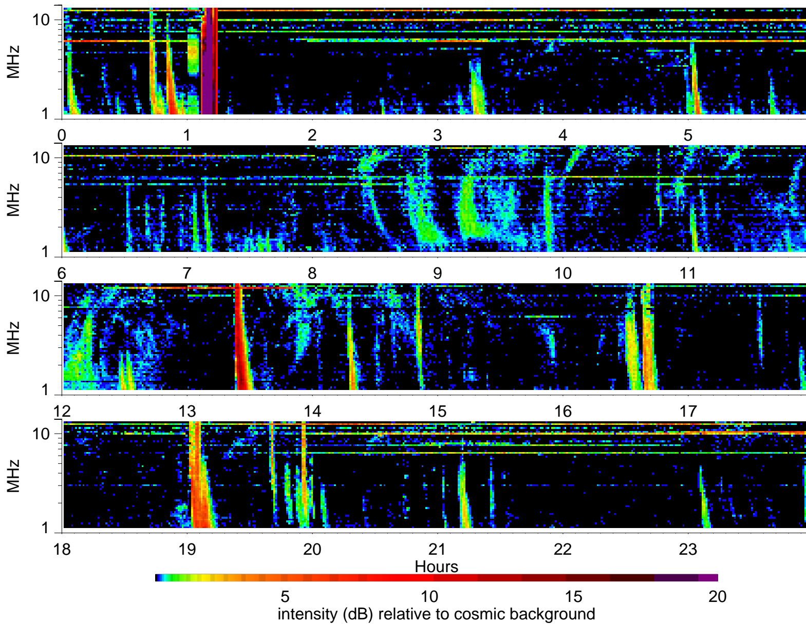
Wind Waves RAD2 receiver: 2000/10/6
