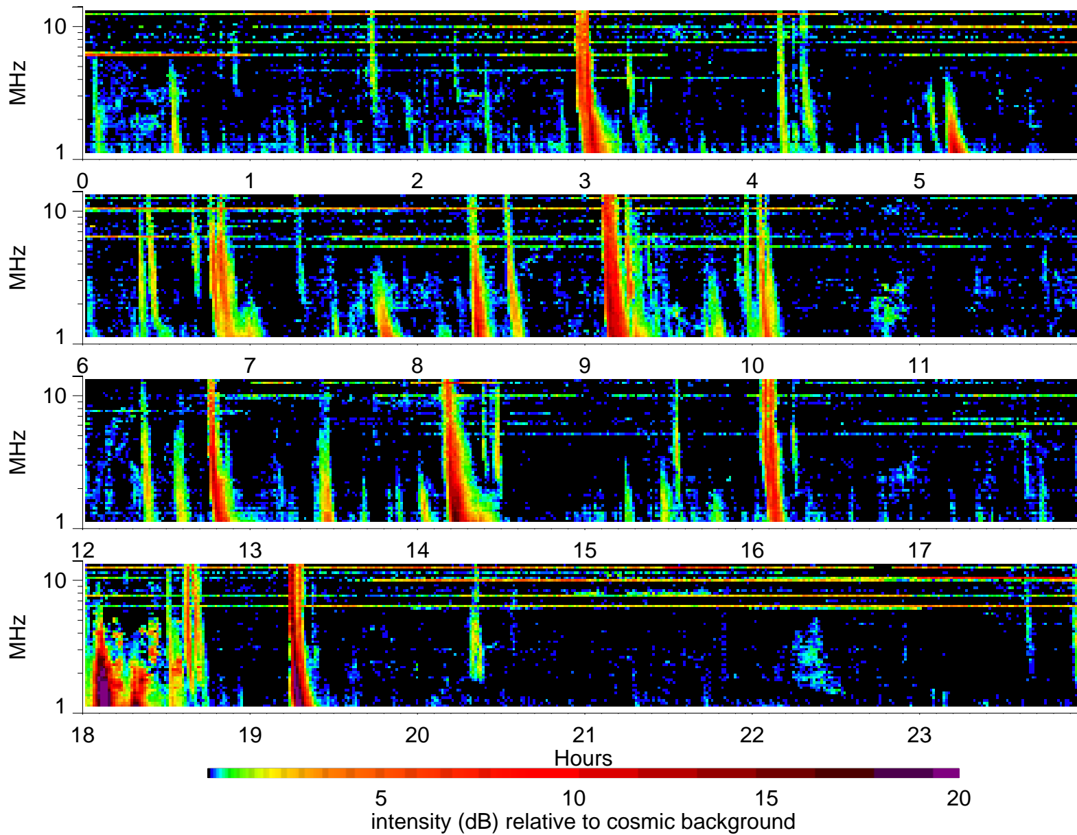
Wind Waves RAD2 receiver: 2000/10/5
