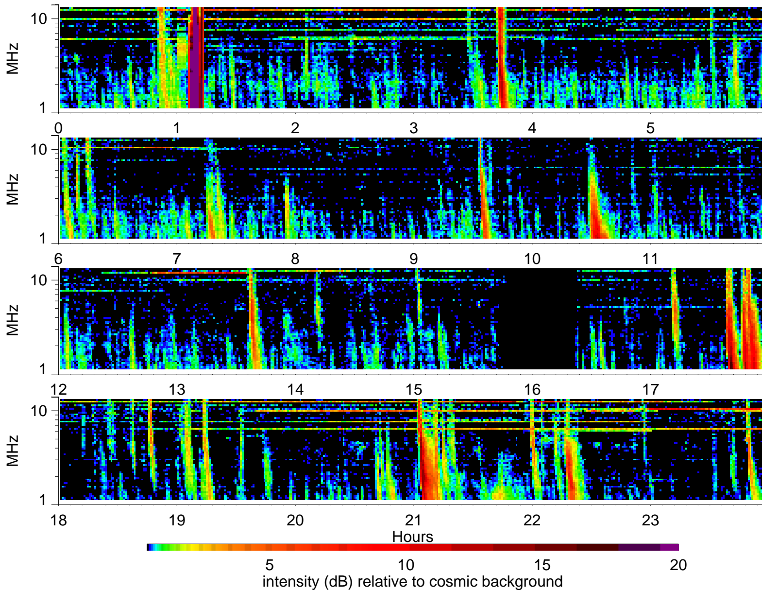
Wind Waves RAD2 receiver: 2000/10/4
