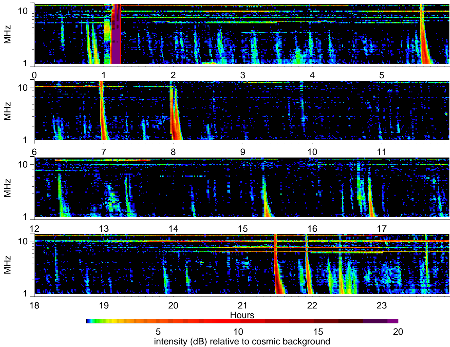
Wind Waves RAD2 receiver: 2000/9/30
