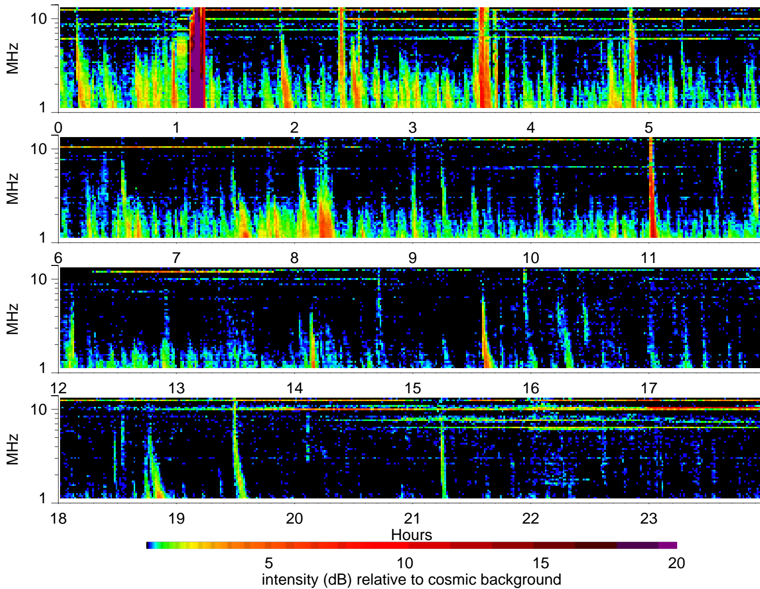
Wind Waves RAD2 receiver: 2000/9/28
