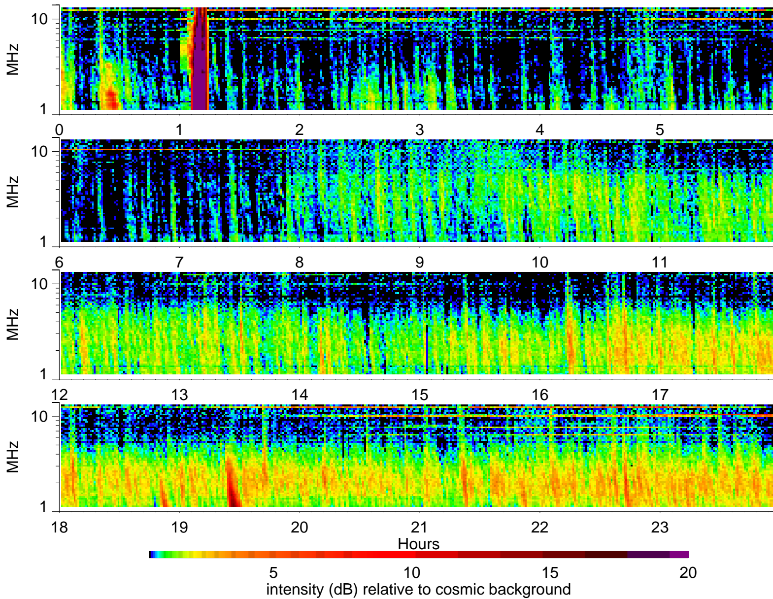
Wind Waves RAD2 receiver: 2000/9/24
