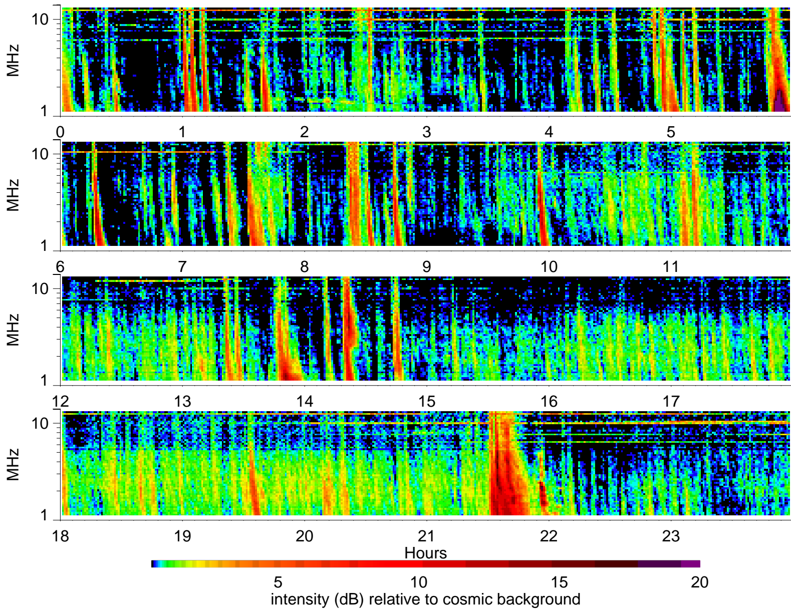
Wind Waves RAD2 receiver: 2000/9/23
