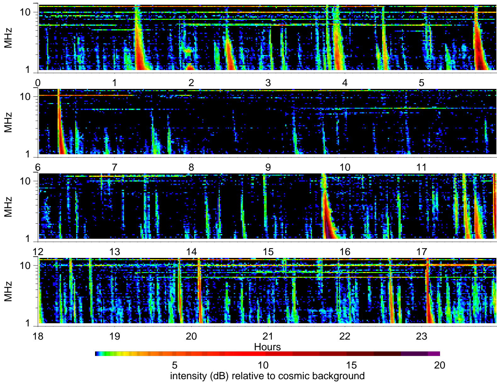
Wind Waves RAD2 receiver: 2000/9/21
