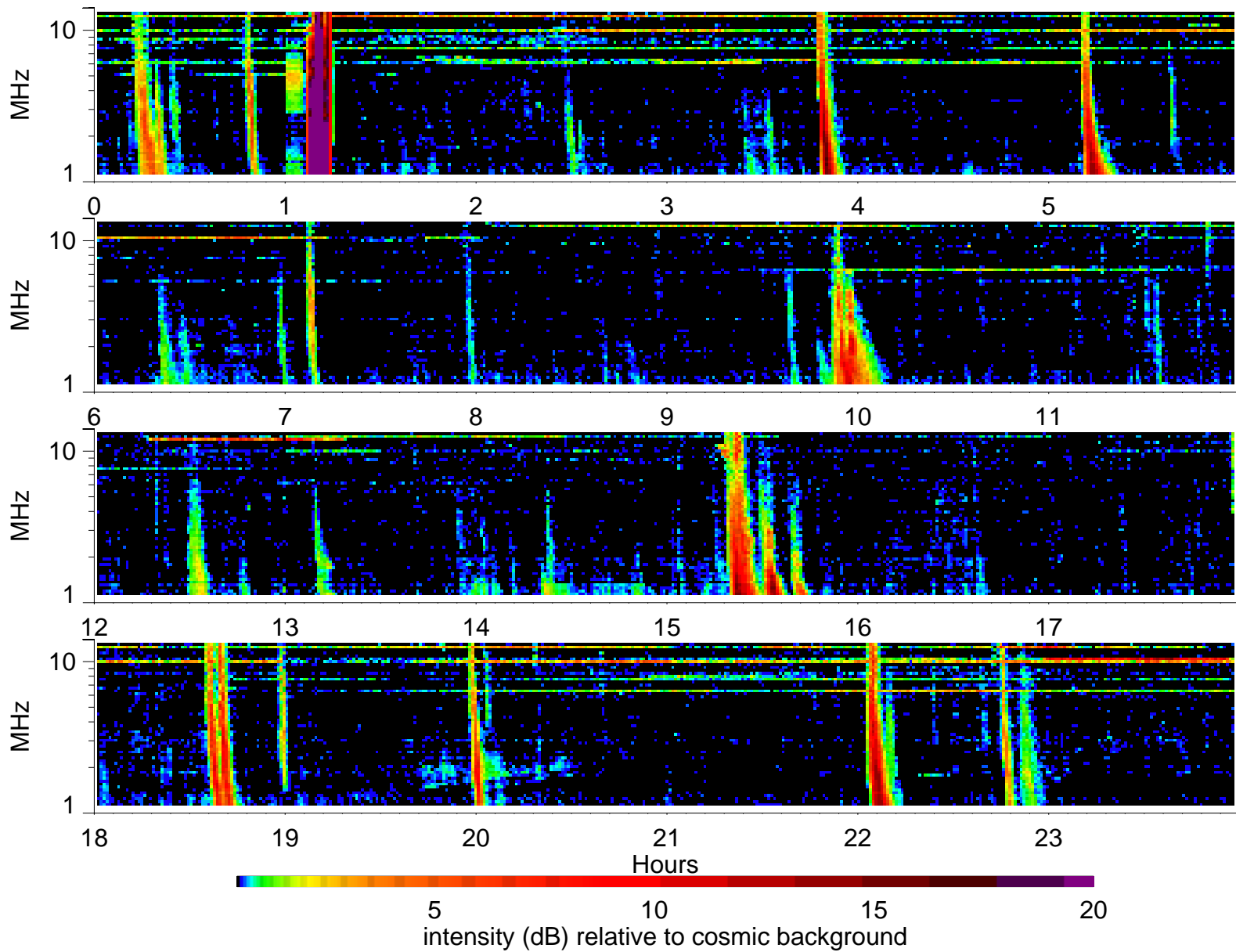
Wind Waves RAD2 receiver: 2000/9/20
