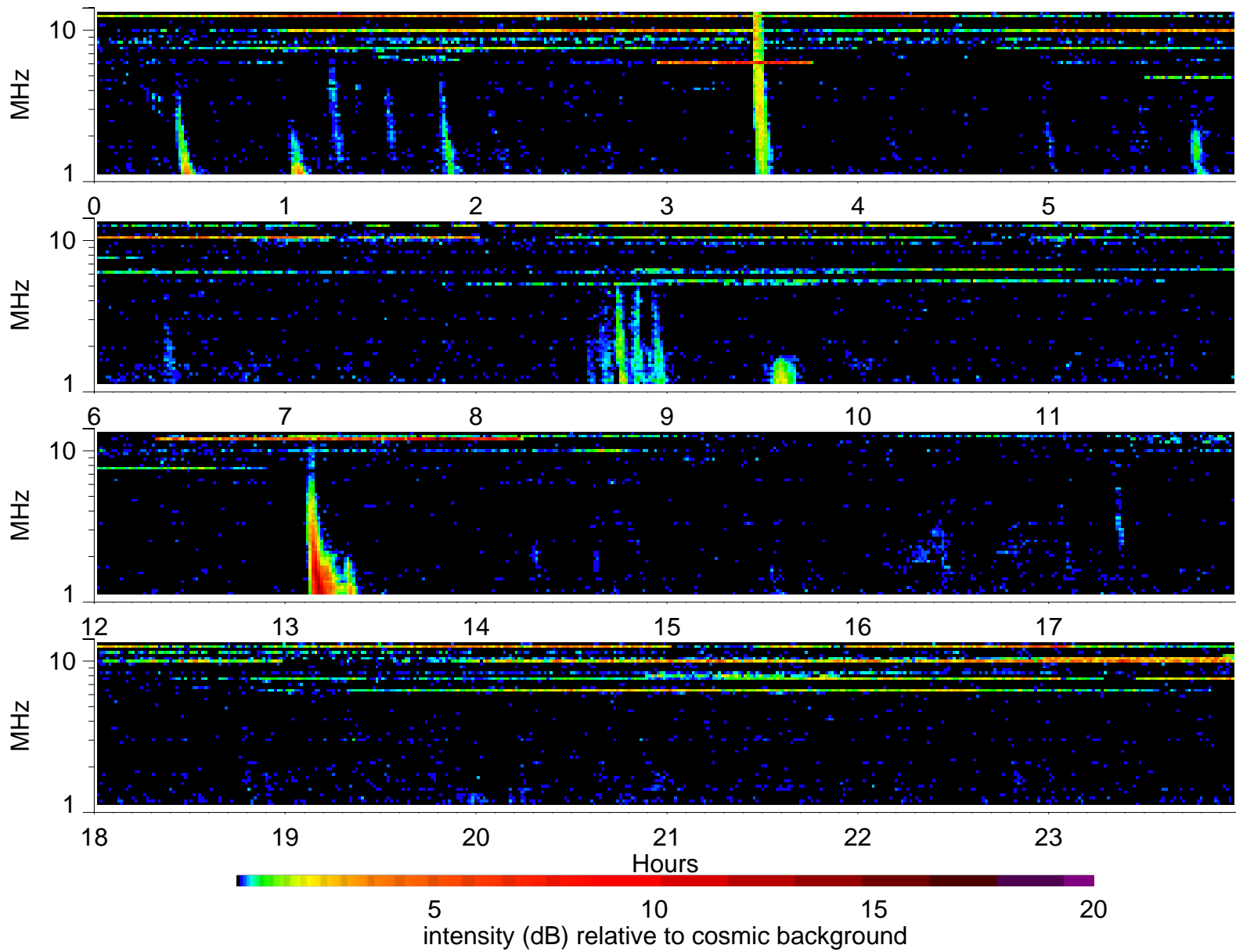
Wind Waves RAD2 receiver: 2000/9/9
