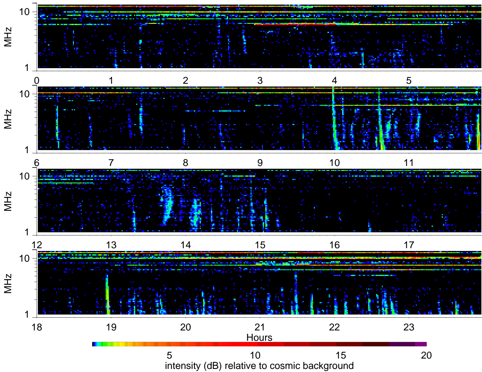
Wind Waves RAD2 receiver: 2000/9/3
