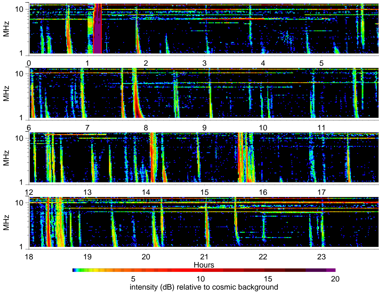
Wind Waves RAD2 receiver: 2000/8/31
