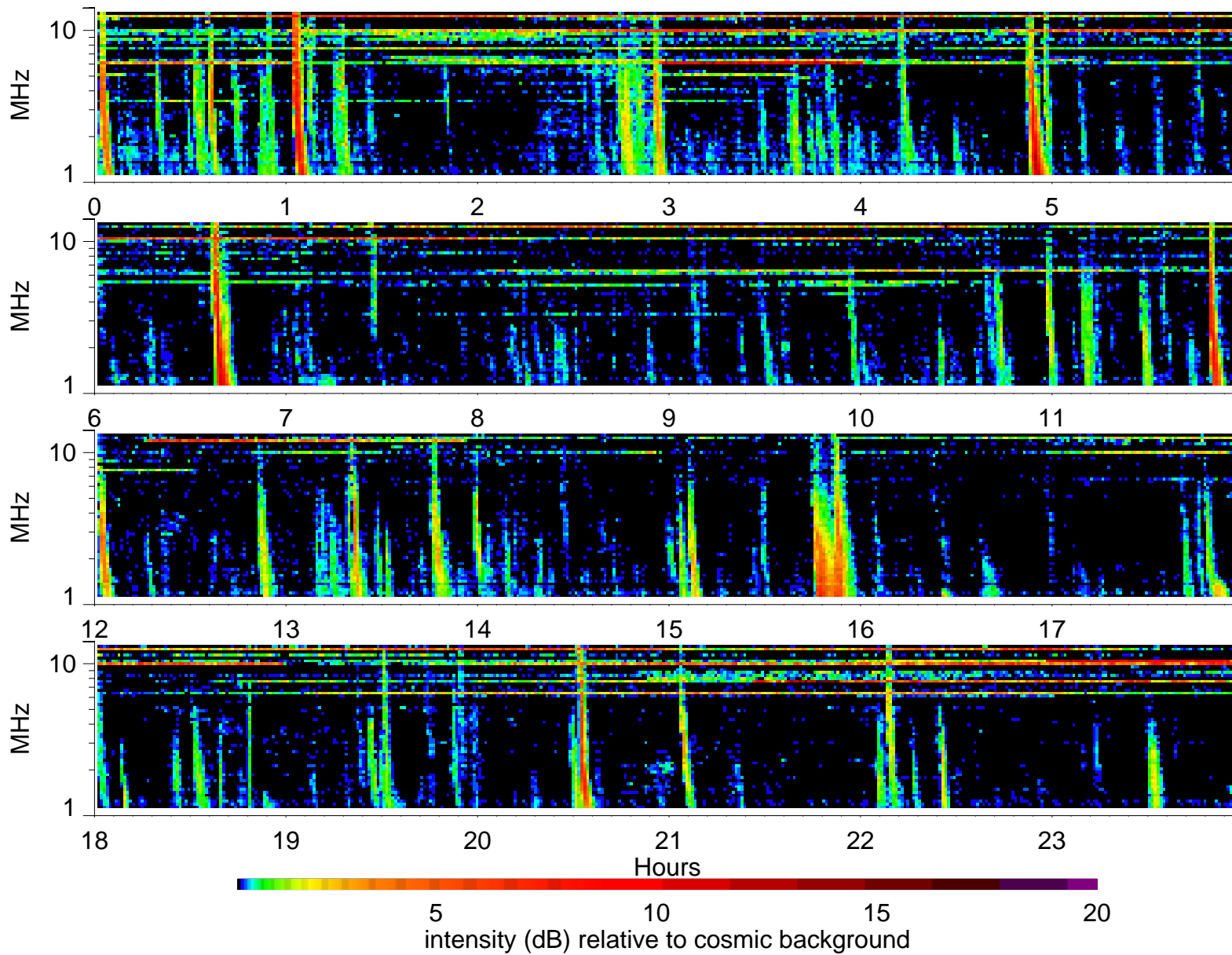
Wind Waves RAD2 receiver: 2000/8/30
