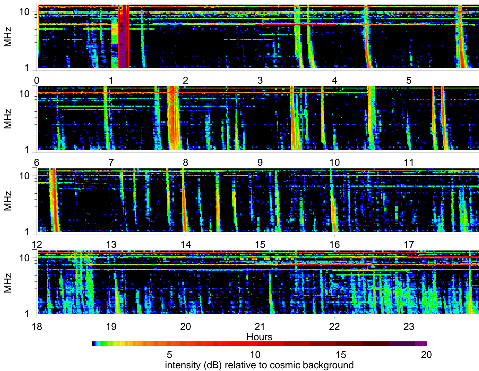
Wind Waves RAD2 receiver: 2000/8/29
