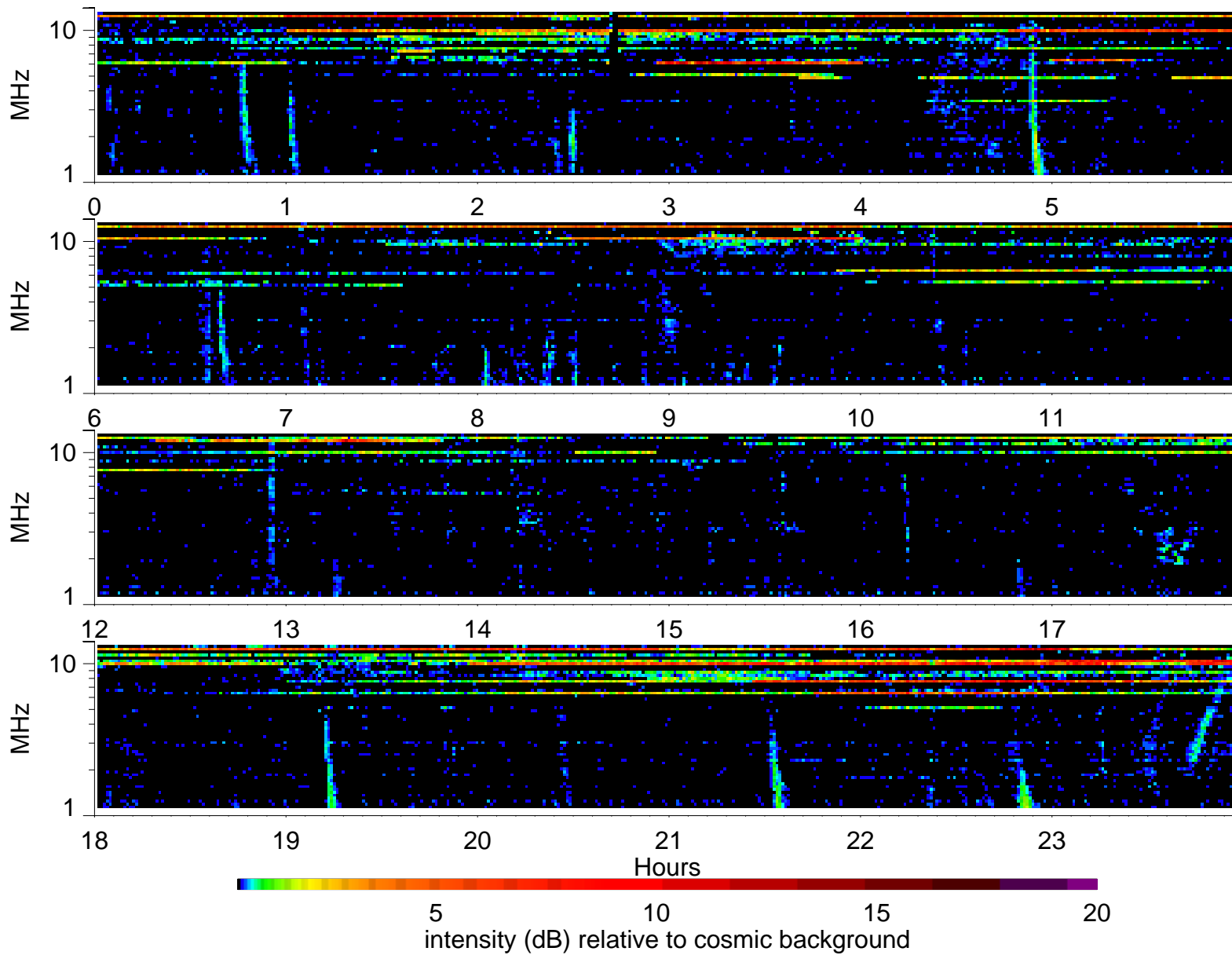
Wind Waves RAD2 receiver: 2000/8/24
