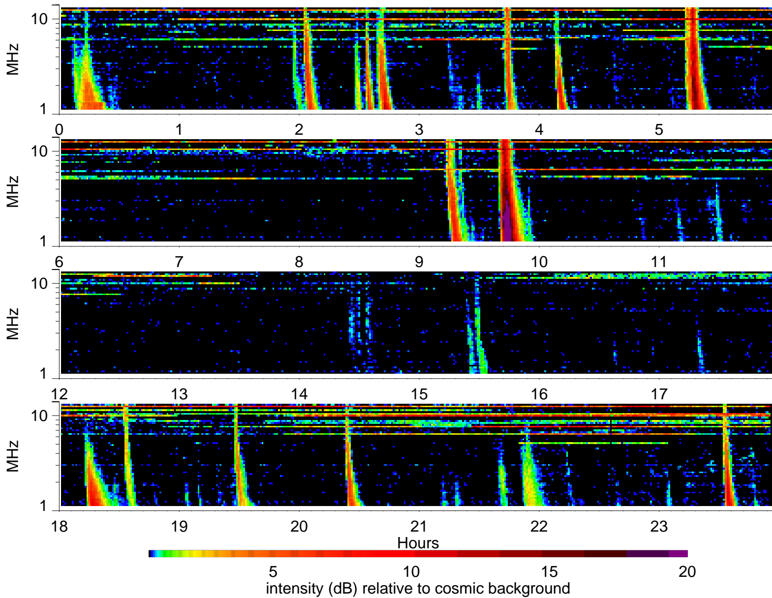
Wind Waves RAD2 receiver: 2000/8/22
