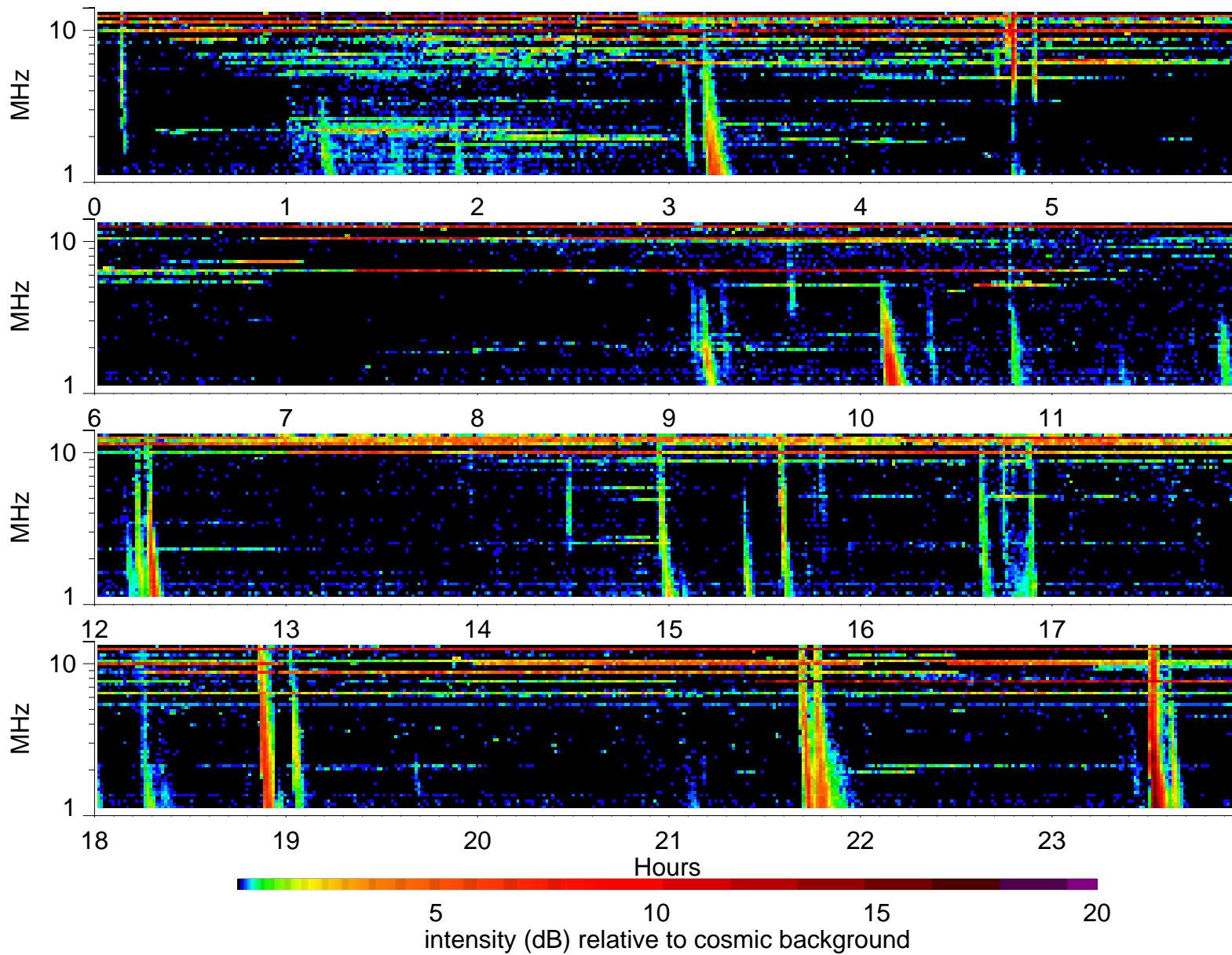
Wind Waves RAD2 receiver: 2000/8/16
