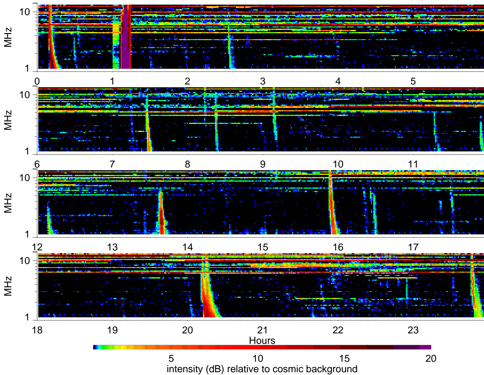
Wind Waves RAD2 receiver: 2000/8/13
