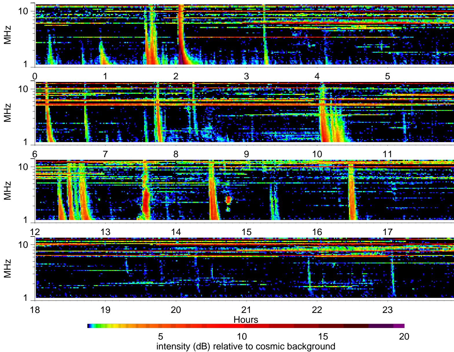
Wind Waves RAD2 receiver: 2000/8/12
