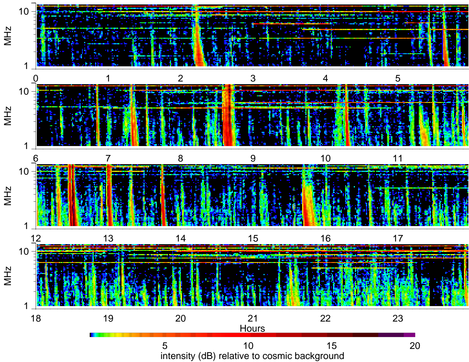
Wind Waves RAD2 receiver: 2000/8/8
