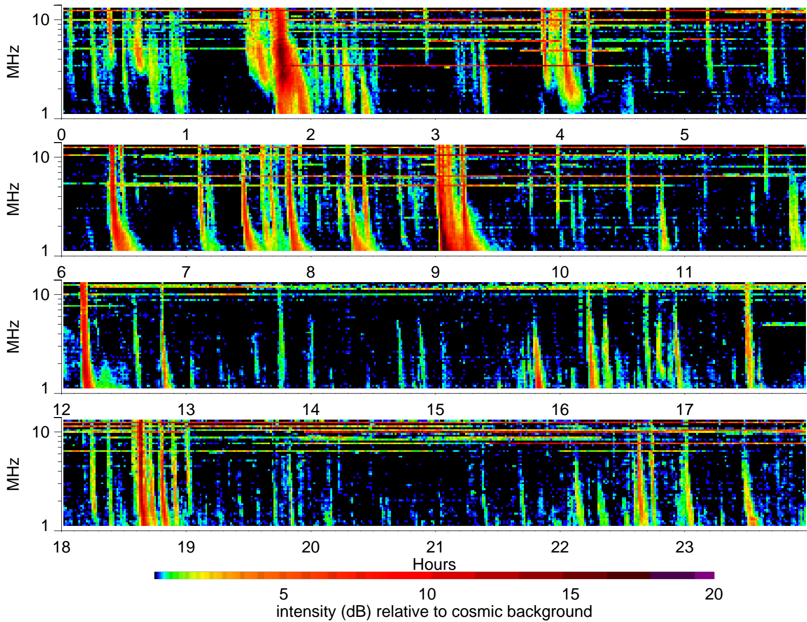
Wind Waves RAD2 receiver: 2000/8/7
