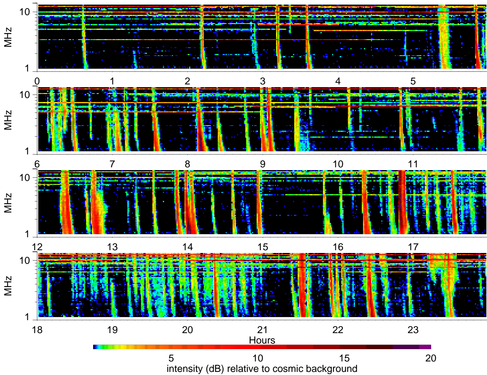
Wind Waves RAD2 receiver: 2000/8/6
