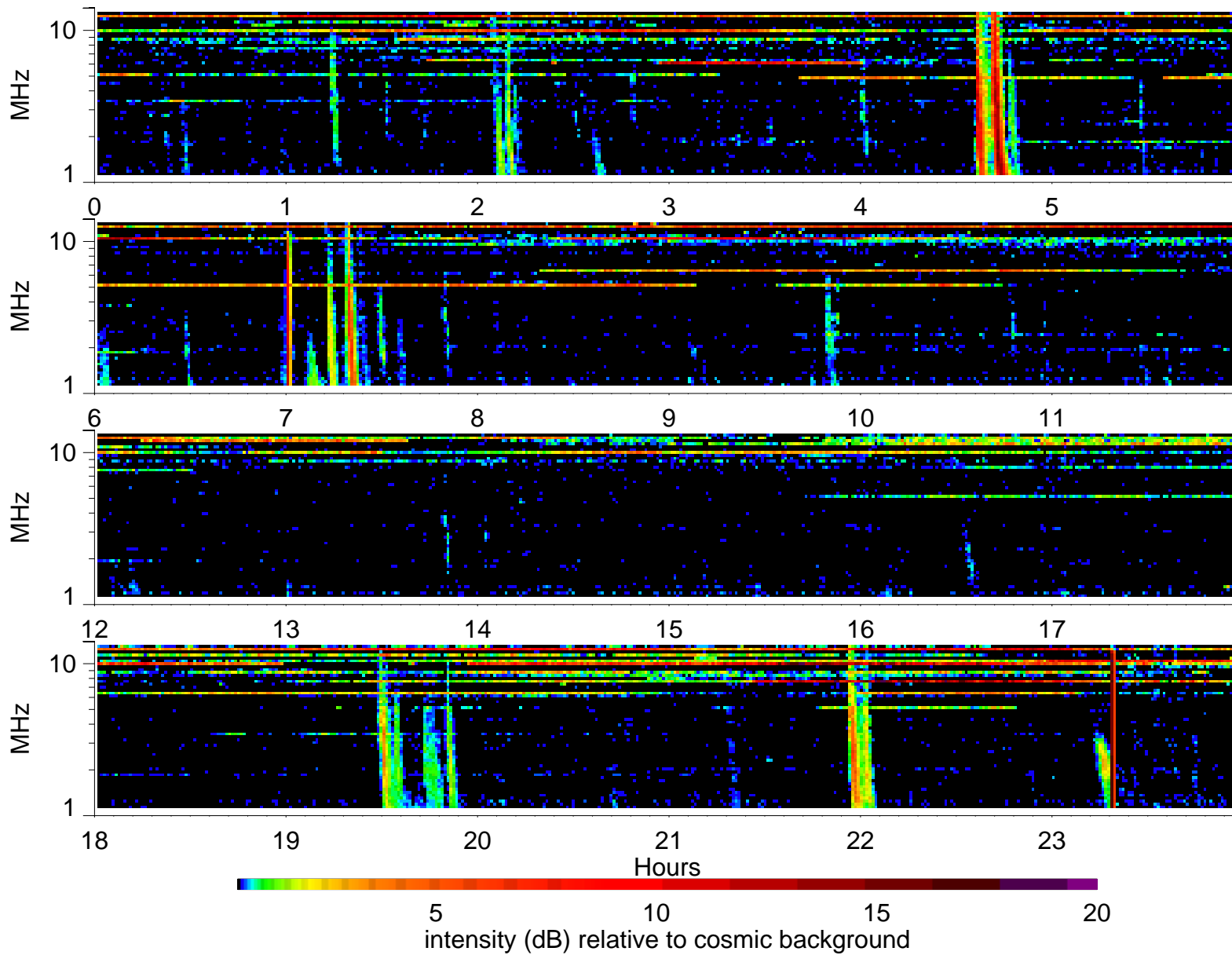
Wind Waves RAD2 receiver: 2000/7/27
