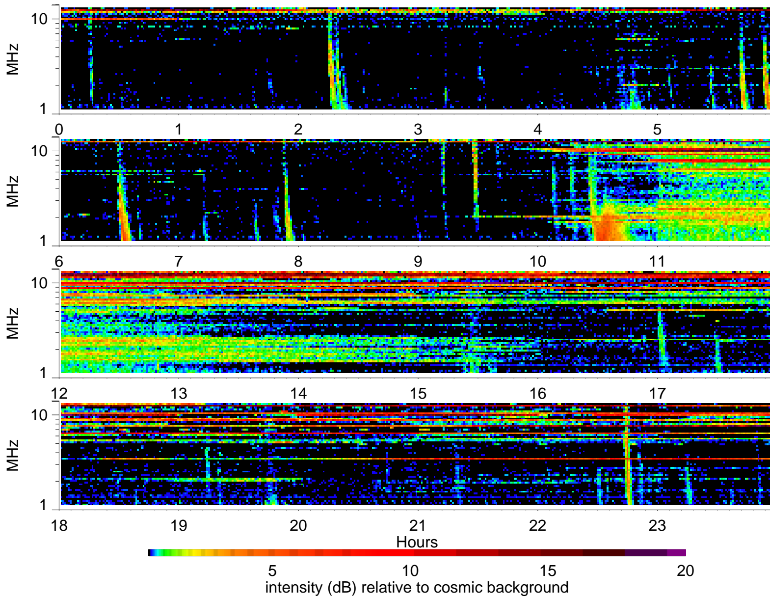
Wind Waves RAD2 receiver: 2000/7/23
