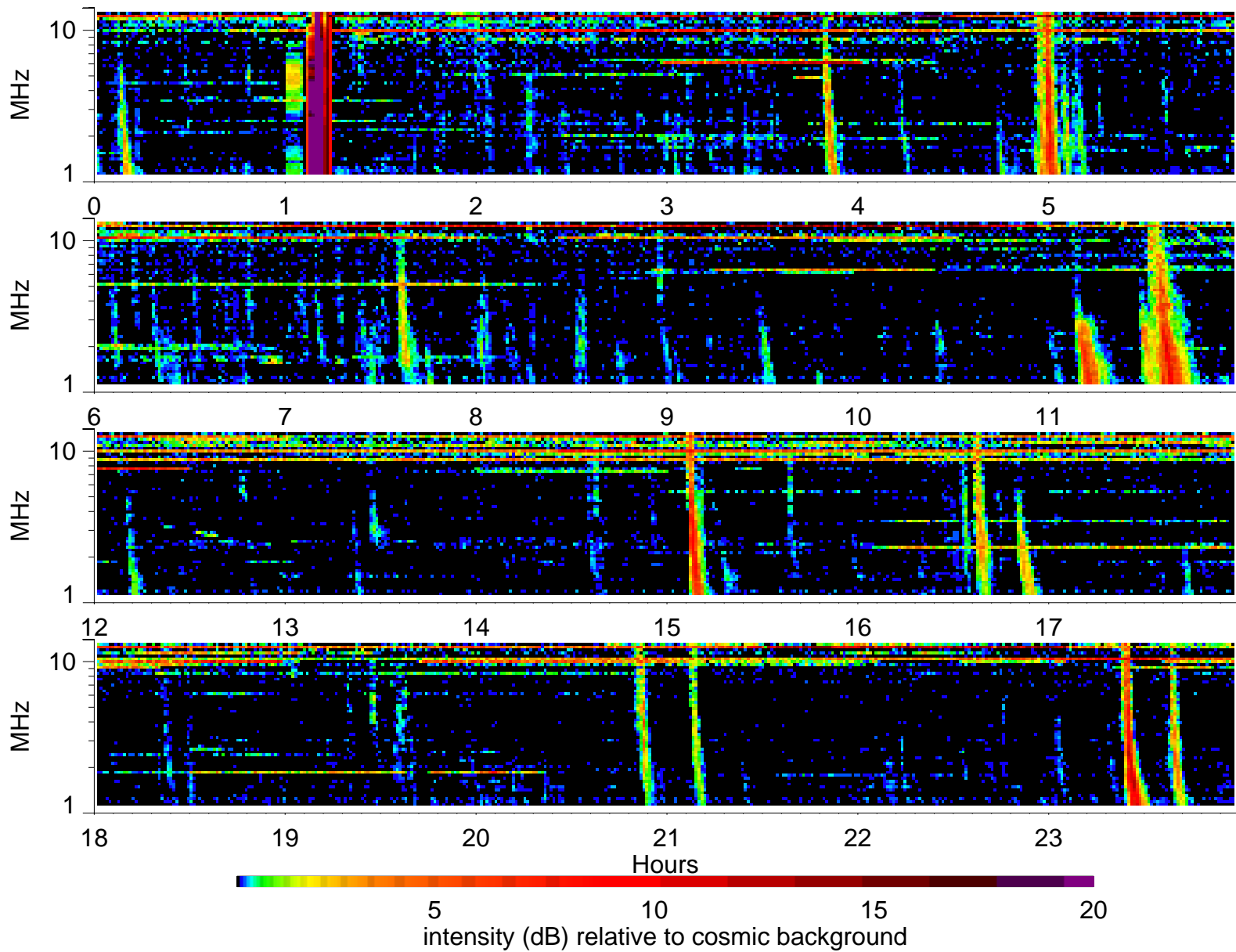
Wind Waves RAD2 receiver: 2000/7/22
