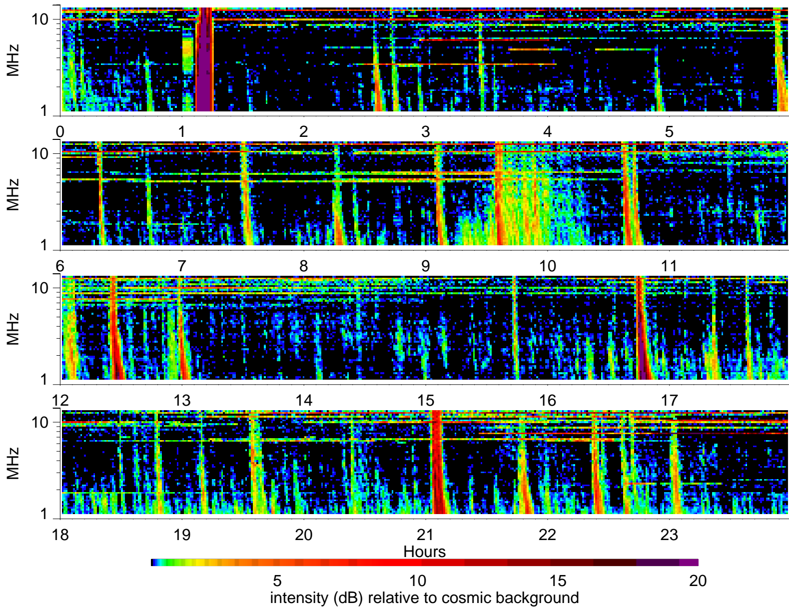
Wind Waves RAD2 receiver: 2000/7/20
