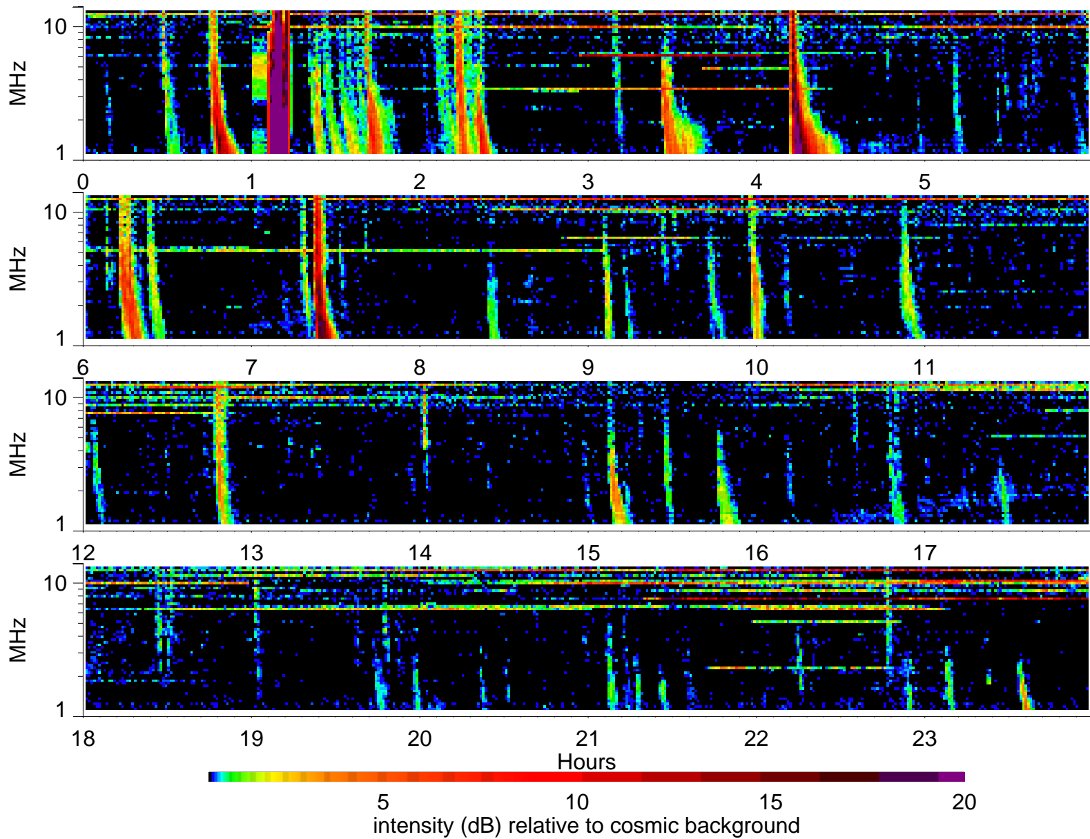
Wind Waves RAD2 receiver: 2000/7/18
