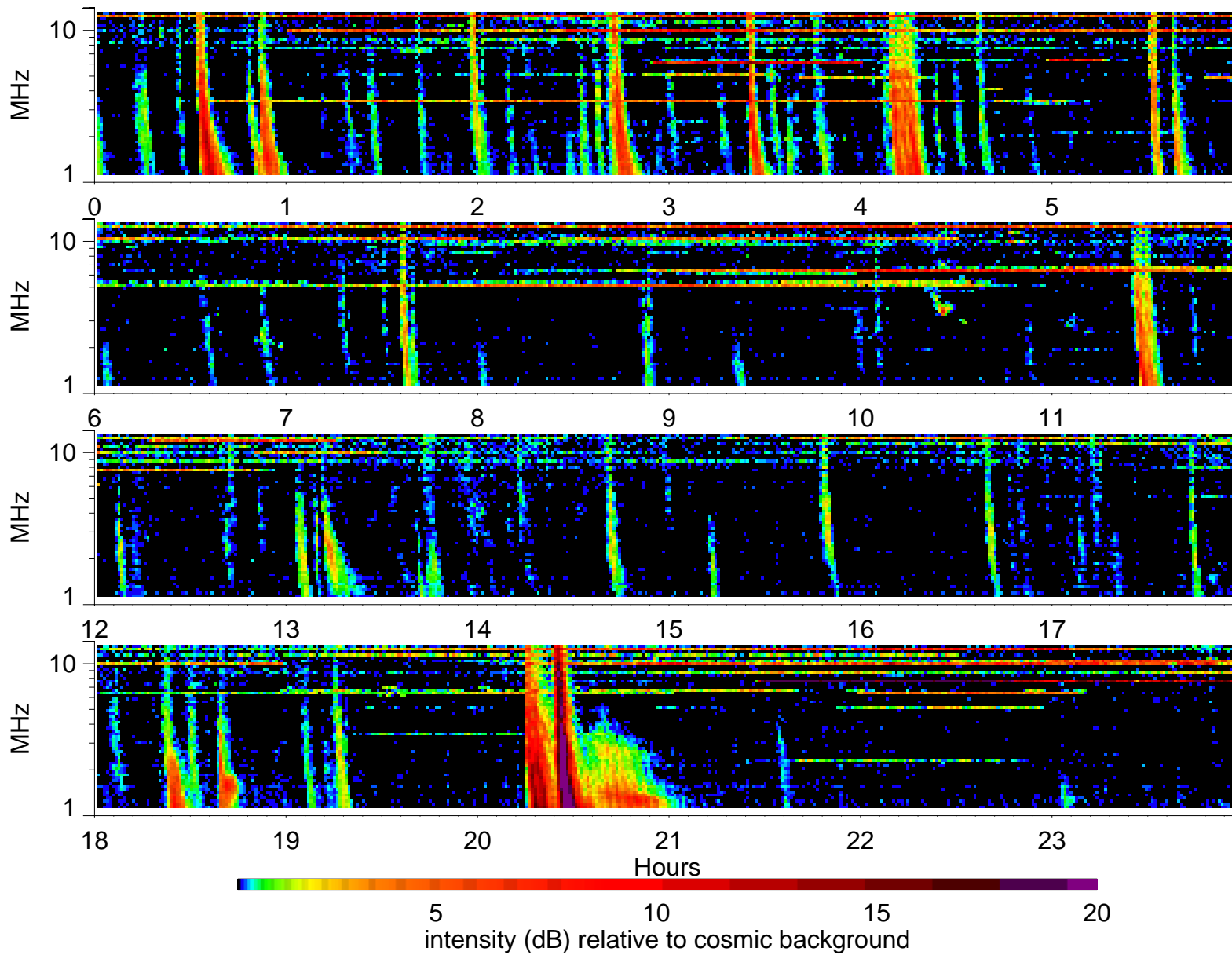
Wind Waves RAD2 receiver: 2000/7/17
