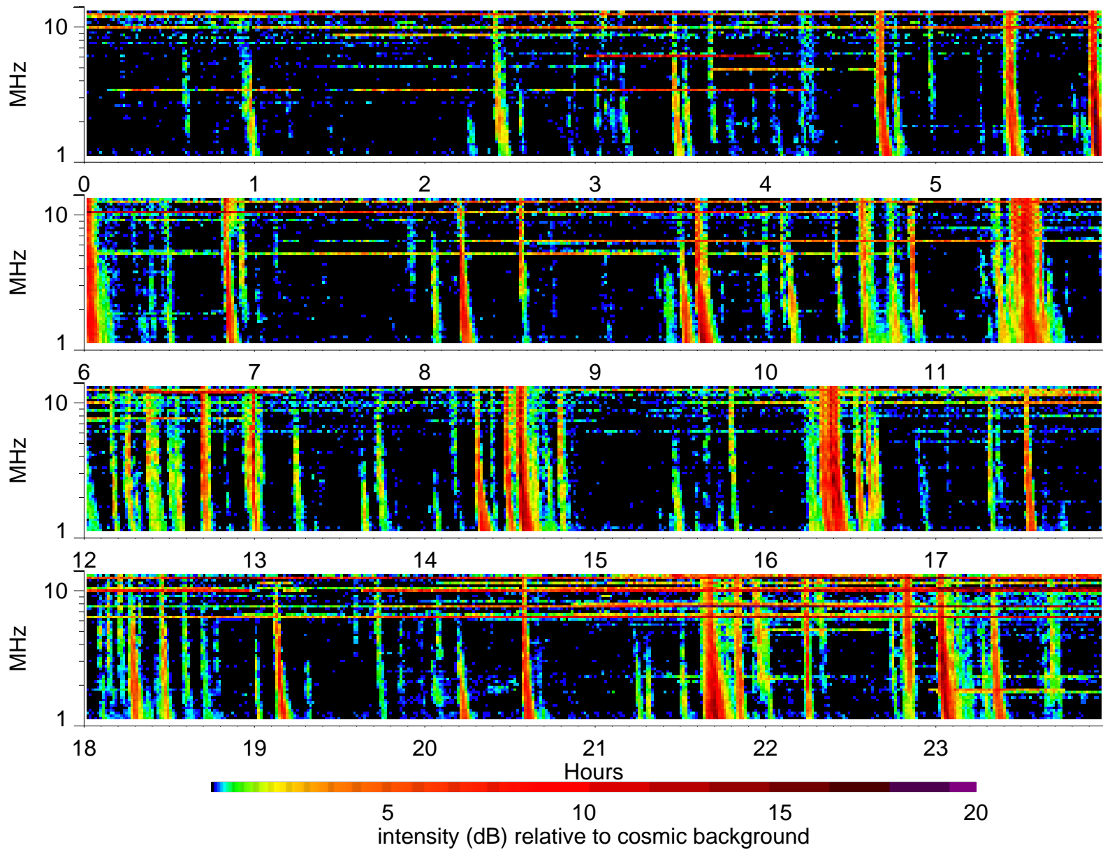
Wind Waves RAD2 receiver: 2000/7/15
