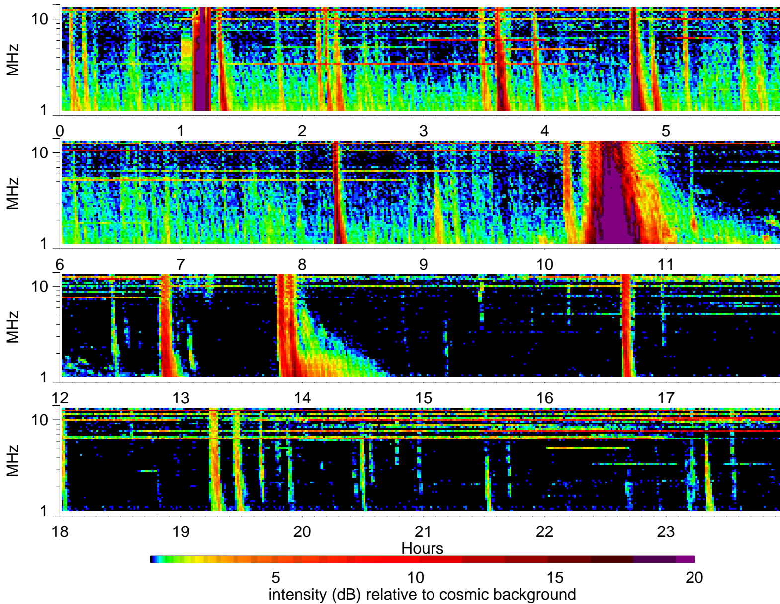
Wind Waves RAD2 receiver: 2000/7/14
