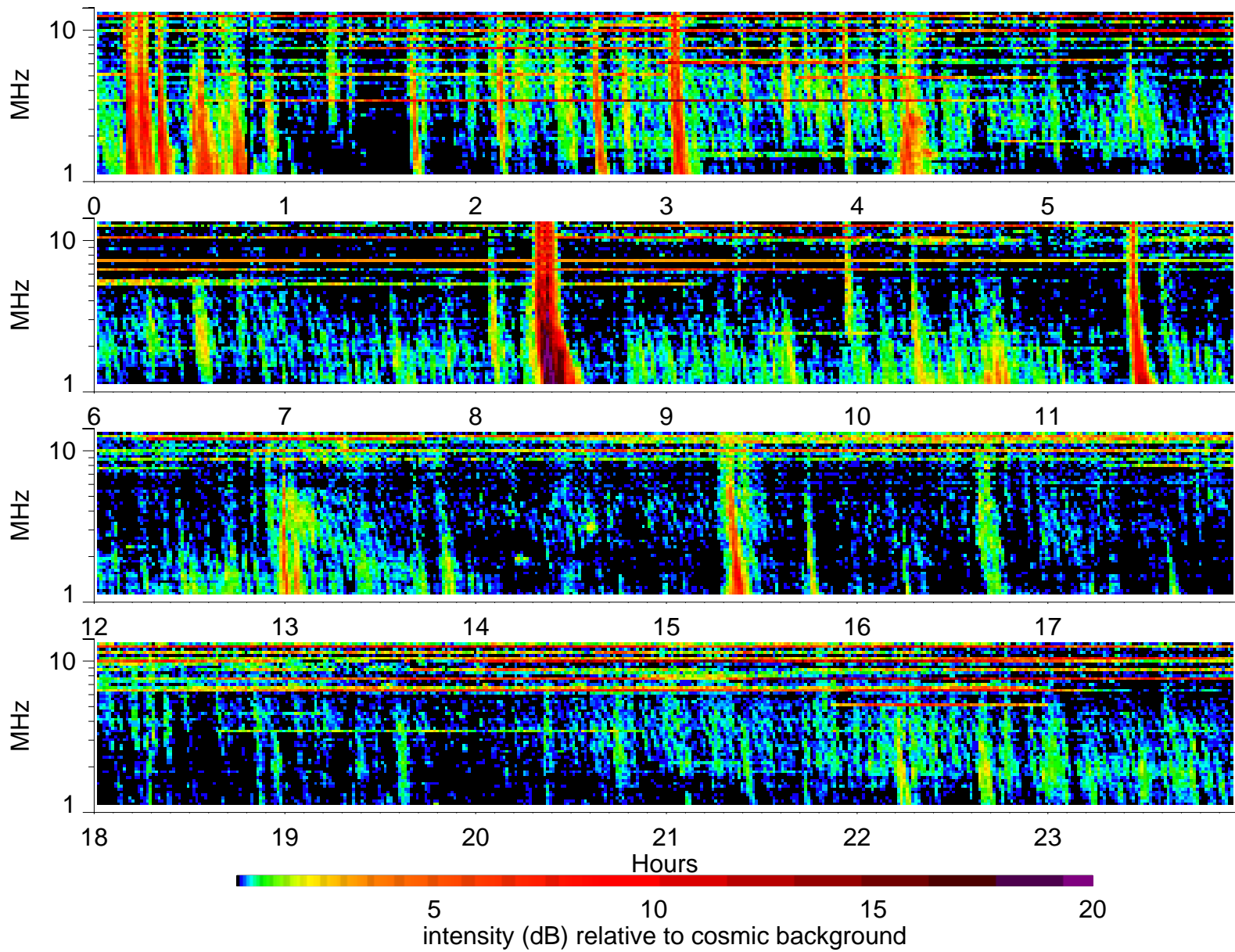
Wind Waves RAD2 receiver: 2000/7/11
