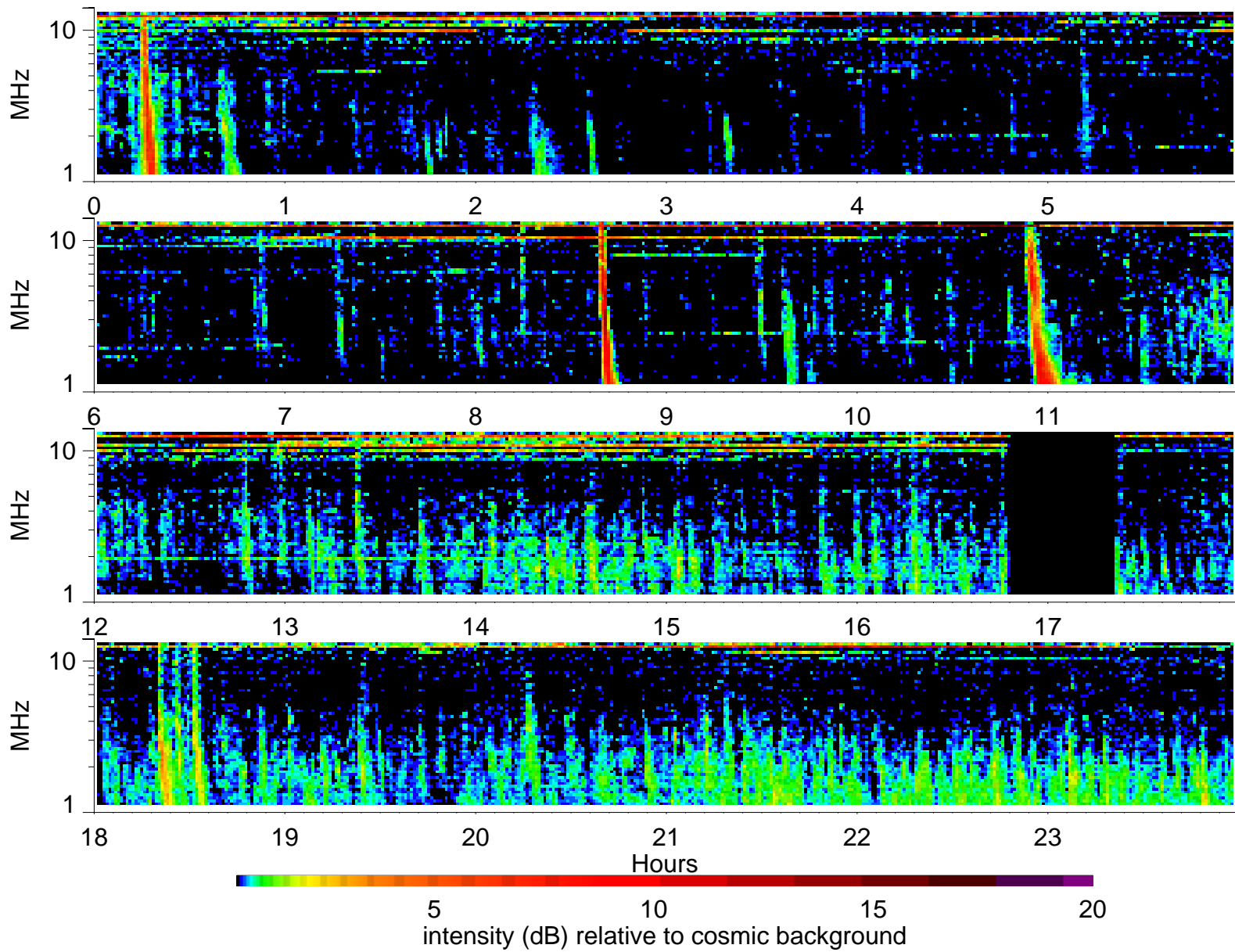
Wind Waves RAD2 receiver: 2000/7/9
