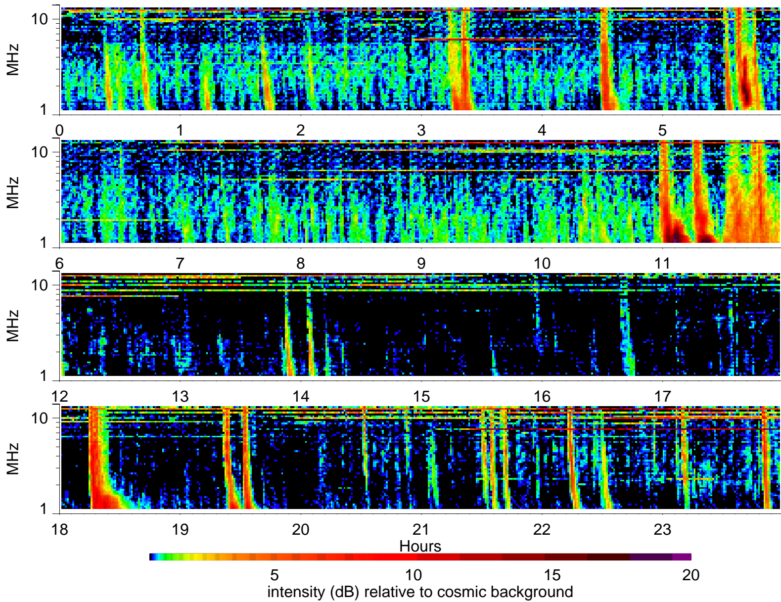
Wind Waves RAD2 receiver: 2000/7/7
