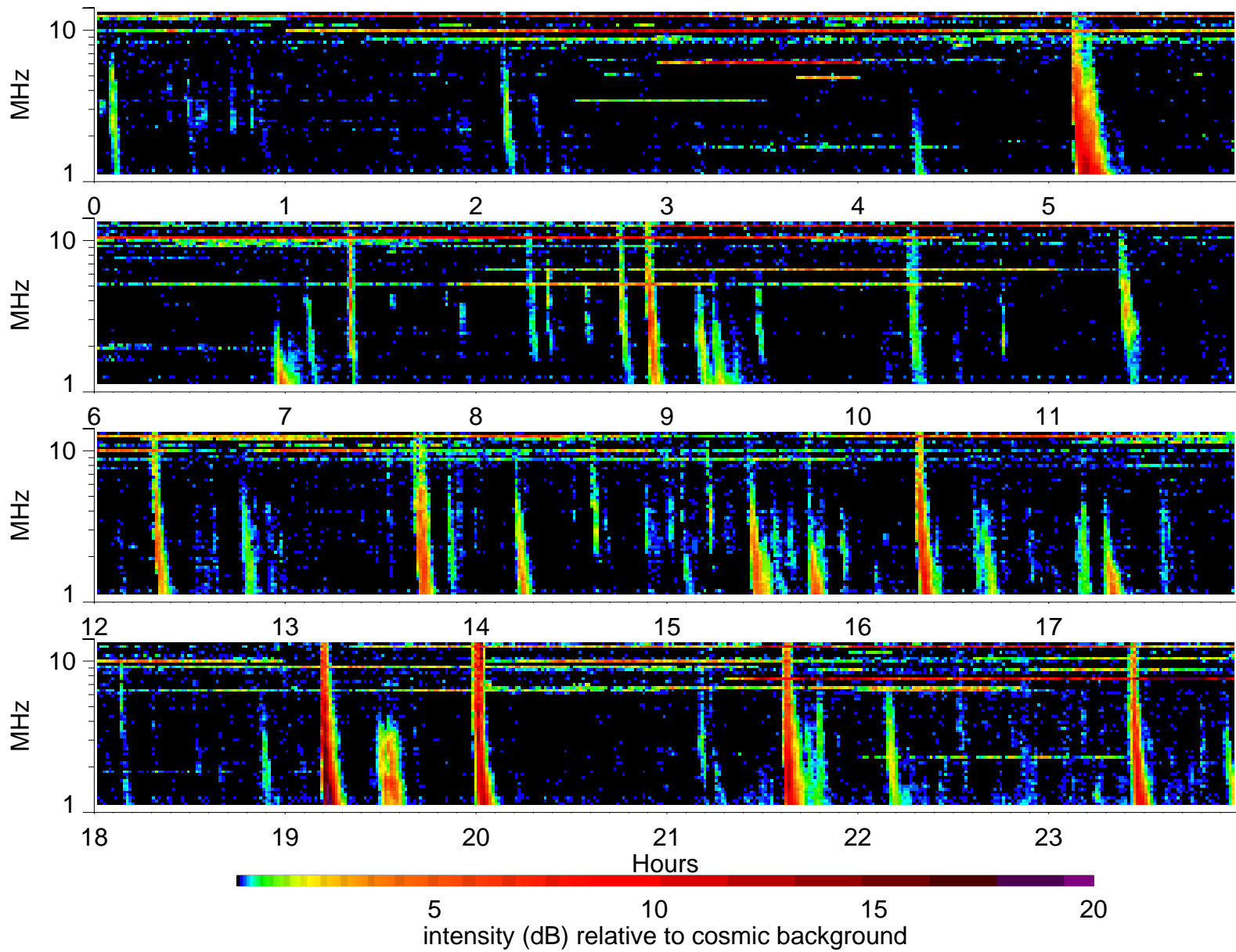
Wind Waves RAD2 receiver: 2000/7/5
