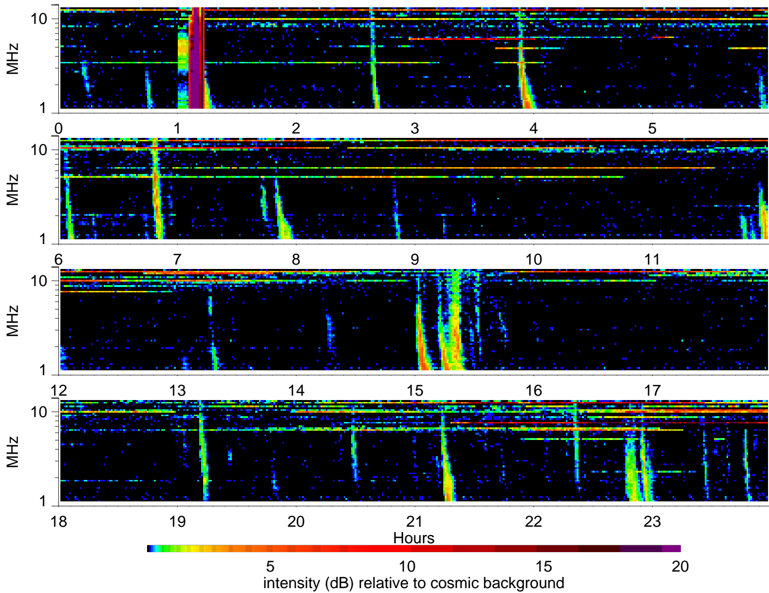
Wind Waves RAD2 receiver: 2000/7/4
